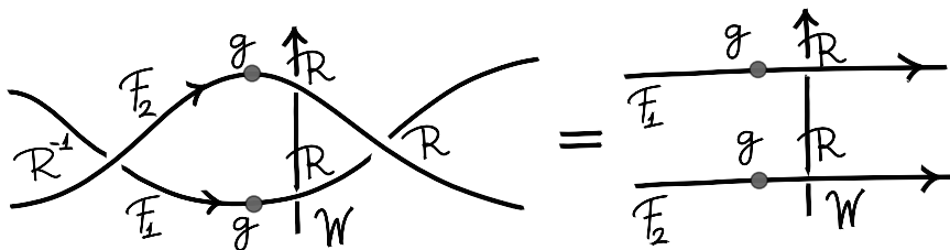
FIGURE 1. From the YB equation and [g \otimes g, R] = 0 we deduce that R_{F_2, F_1} conjugates g_{F_2} R_{F_2, W} g_{F_1} R_{F_1, W} to the product in the opposite order. Taking the trace over F_2 \otimes F_1 gives (1.5).
