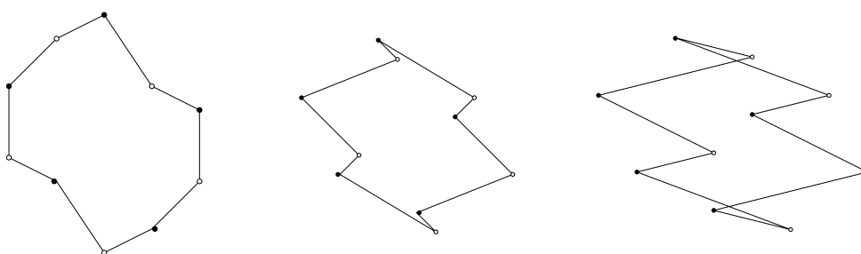
FIGURE 1.4. The singularity \circ is moved to the right with respect to \bullet , and the picture becomes nonsensical.
