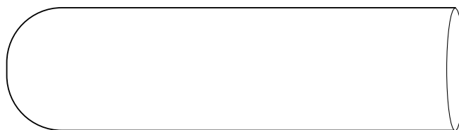
FIGURE 1.1. A cigar-shaped warped product.
