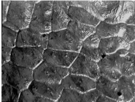
FIGURE 1. Grains in aluminum: a typical grain size is around 10 micrometer, the lattice parameter of aluminum amounts to 4.05 \cdot 10^{-7}\text{m} .
