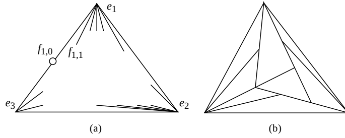
FIGURE 1. (a) Three Newton polygons; (b) subdivision into regular triangles
