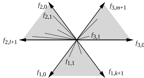
FIGURE 3. “Propellor” with three “blades”
