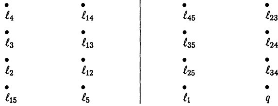
Figure 1 : Graph \Gamma
