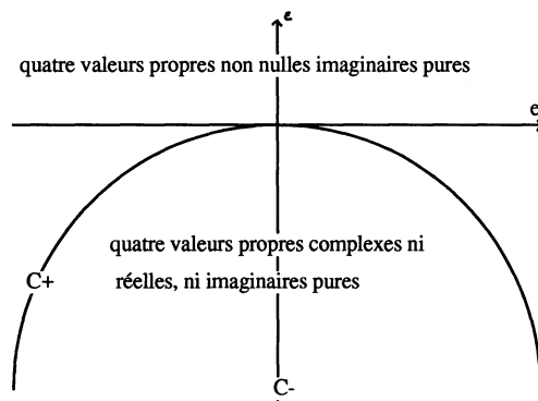
FIGURE 7.2 : \mu_1 = \mu_2 . -
