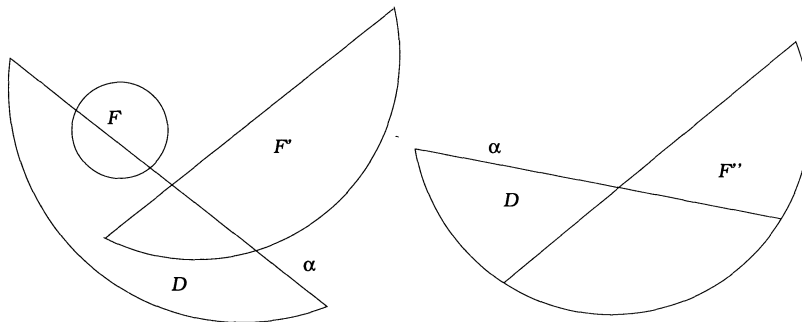
FIGURE 3.2. Various examples of dipping intersections. Loosely speaking \alpha plays the role of the milk surface, F , F' , and F'' the breads, and D^o the milk. The left one indicates nice dippings, and the right one not a nice one.
