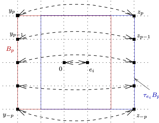
FIGURE 4. Change of variable \widehat{\eta} \rightarrow T_{i,p}^x \widehat{\eta} .
